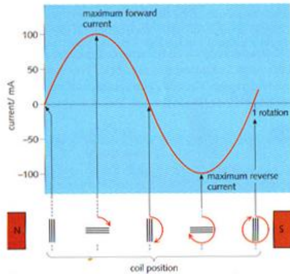
Graph showing the generator's AC output
