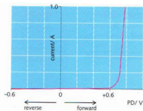
Semiconductor diode The current is not proportional to the PD. And if the PD is reversed, the current is almost zero. In effect, the diode 'blocks' current in the reverse direction.
